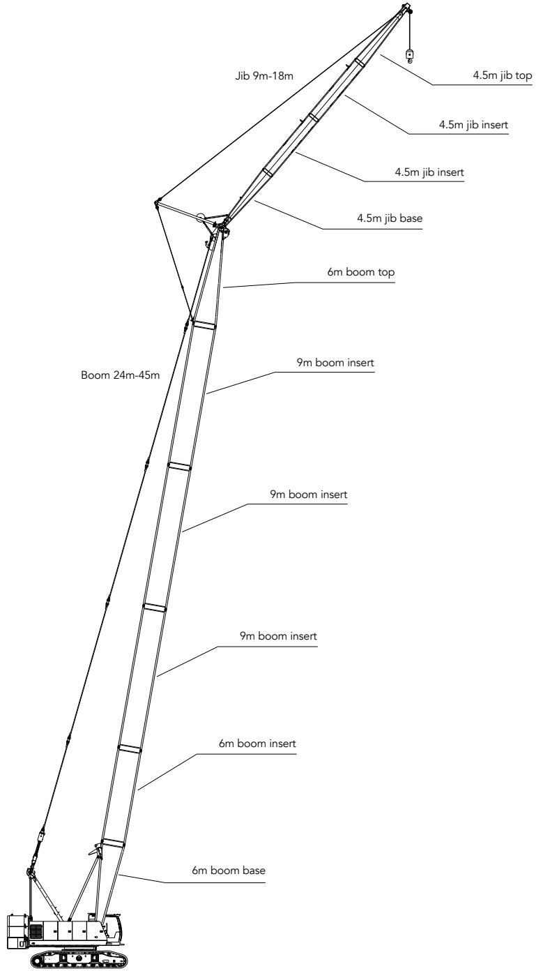
FJ Configuration (Longest boom+ jib: 45m+18m)
